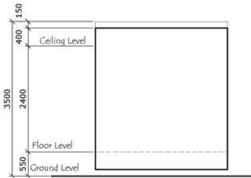
TYPICAL SIDE ELEVATION
