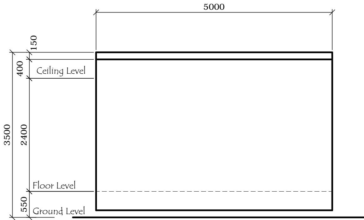
Left Side Elevation (South) SCALE: 1: 50 M
