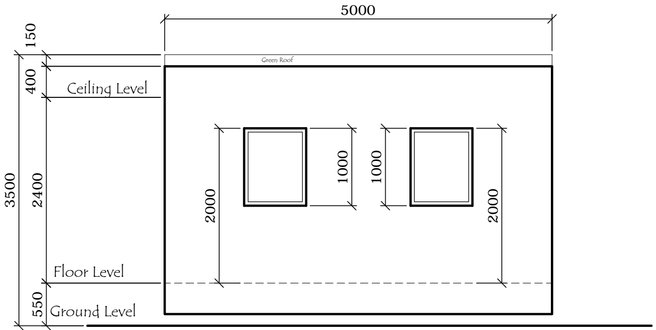
REAR ELEVATION
