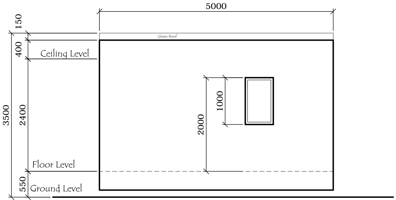
LEFT ELEVATION
