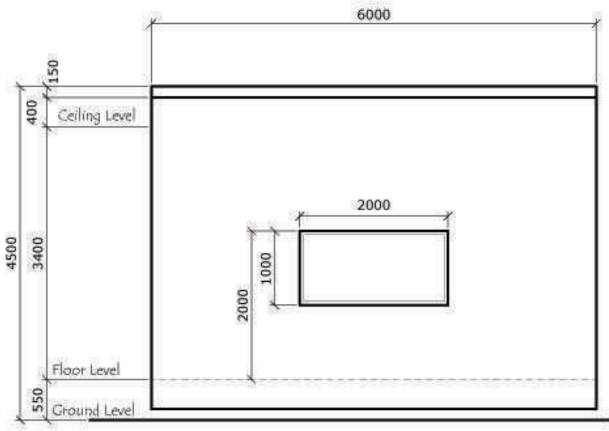
○ Left Side Elevation SCALE: 1:50 M
